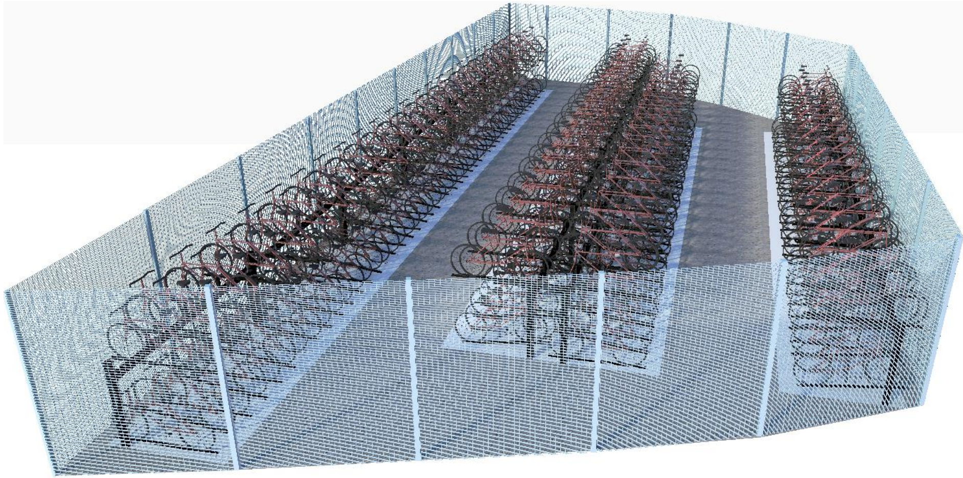
Indicative integral layout of the cycle hub showing 3 lines of cycle racks with circulation for cyclists. Entrances would be on the shorter boundaries of the cycle hub.
